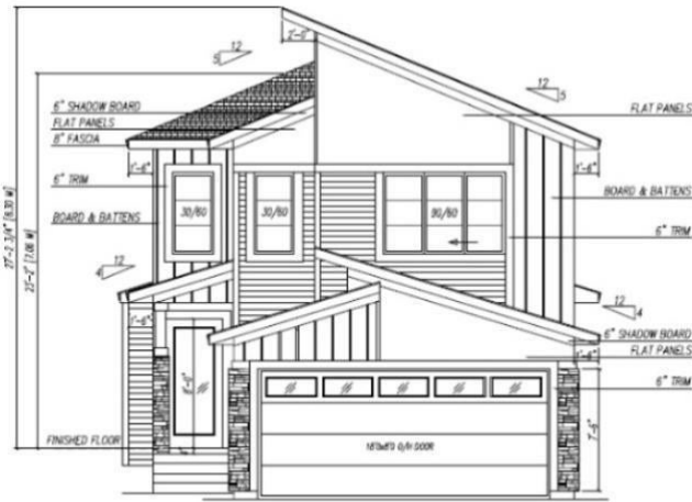
FRONT ELEVATION
